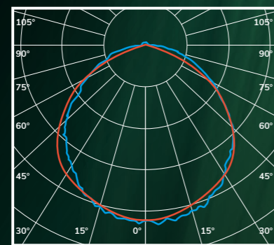
LIGHT DISTRIBUTION WITH OPAL GLOBE
