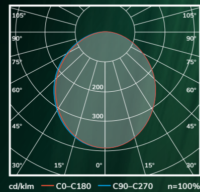
LIGHT DISTRIBUTION WITH OPAL GLOBE
