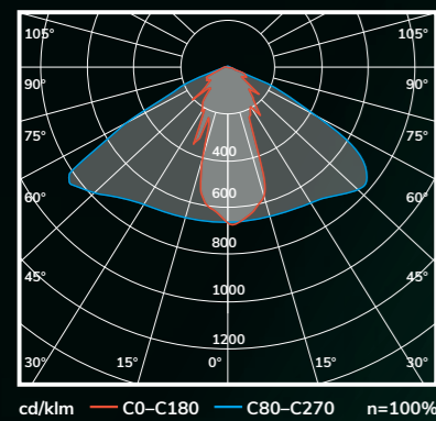
LIGHT DISTRIBUTION WITH LENS GLOBE
